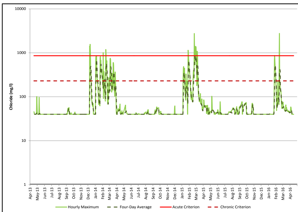
Figure 1-12: Estimated Chloride (mg/l), Long Branch
