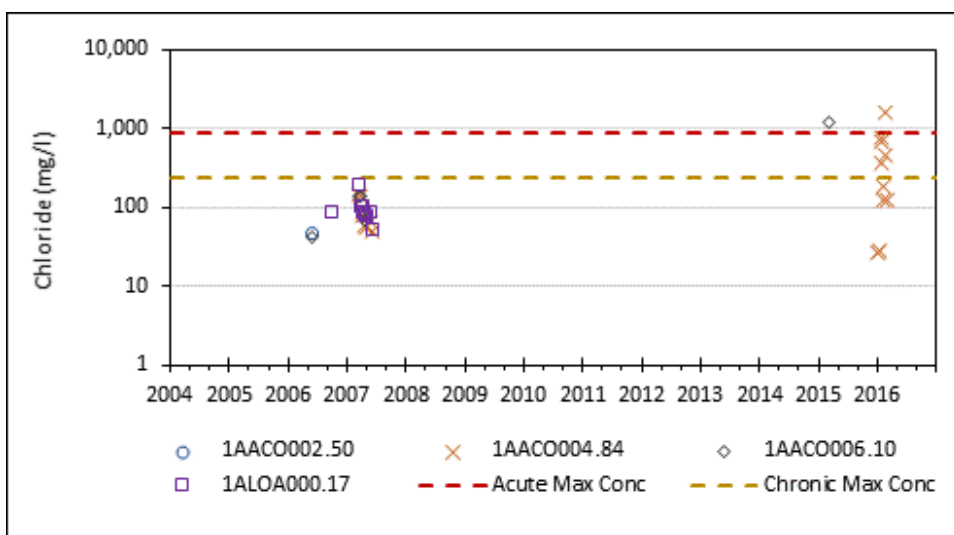
Figure 1-4: Observed Chloride (mg/l) in Lower Accotink Creek
