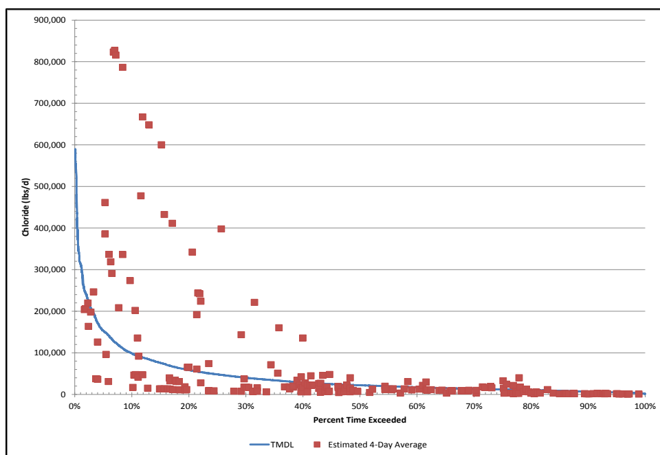
Figure ES-5: Four-Day Average Chloride Load in Extended Winter Season, Accotink Creek near Annandale, with Four-Day Average Chloride Load Estimated from Continuous Specific Conductance Monitoring Data and Linear Regression Model of Chloride-Specific Conductance Relation
