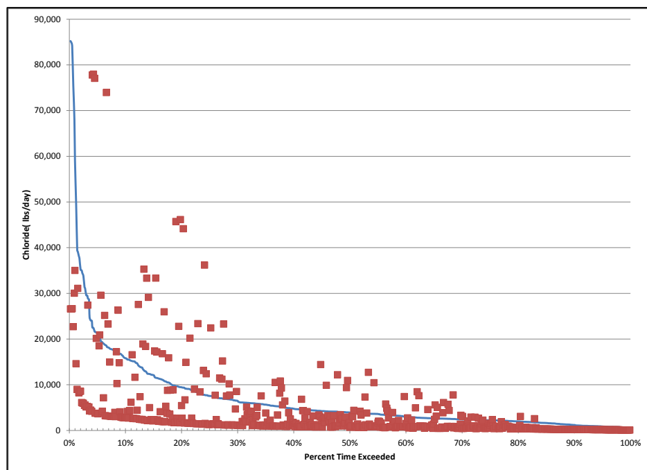
Figure ES-5: Four-Day Average Chloride Load in Extended Winter Season, Accotink Creek near Annandale, with Four-Day Average Chloride Load Estimated from Continuous Specific Conductance Monitoring Data and Linear Regression Model of Chloride-Specific Conductance Relation
