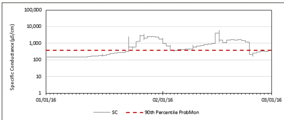
Figure 3-44: Observed Specific Conductance ( \mu\text{S}/\text{cm} ), Continuous Monitoring, Accotink Creek near Telegraph Road
