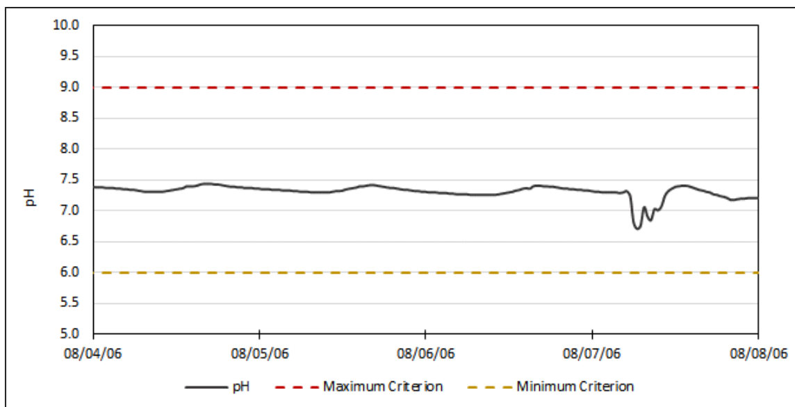
Figure 3-26: Observed pH, Continuous Monitoring, Accotink Creek at Alban Road
