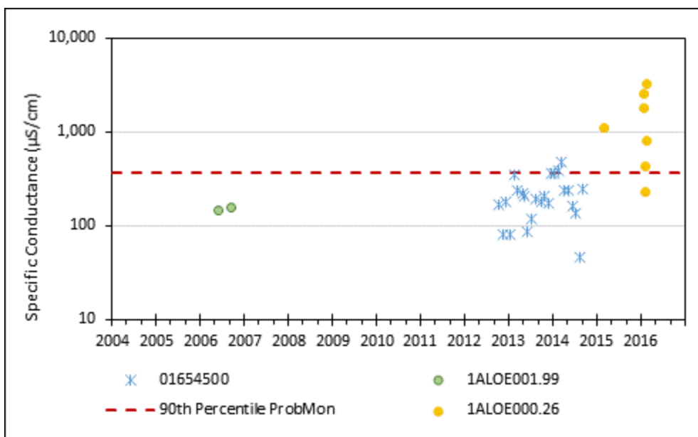
Figure 3-37: Observed Specific Conductance (µS/cm) in Long Branch
