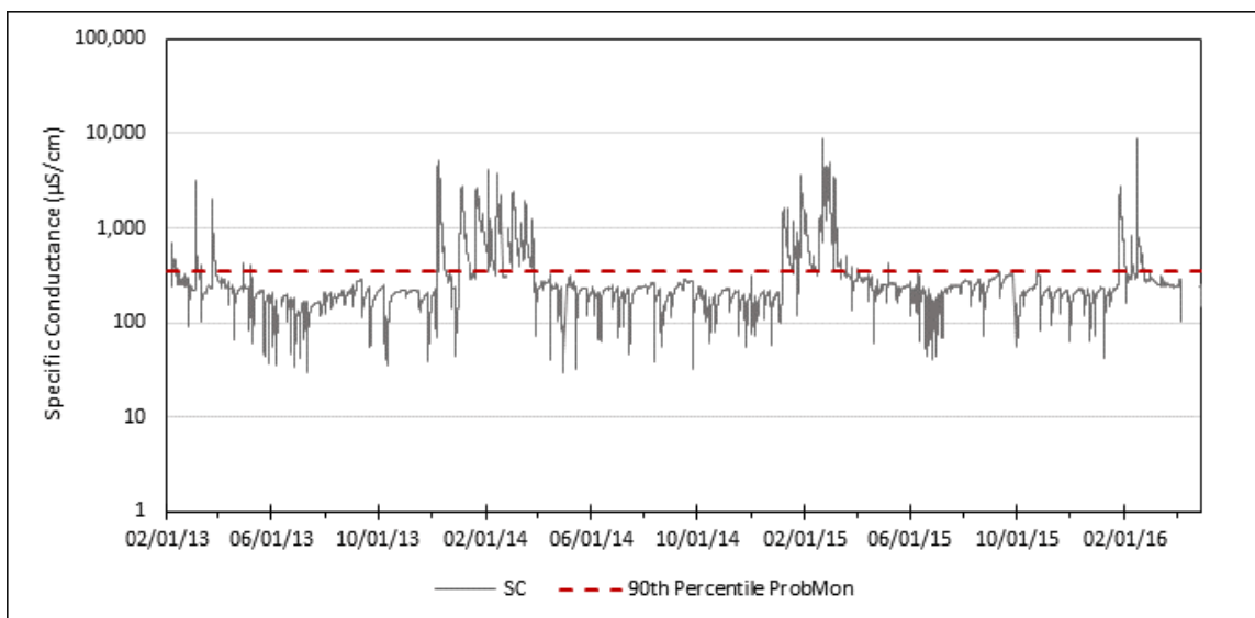
Figure 3-42: Observed Specific Conductance ( \mu\text{S/cm} ), Continuous Monitoring, Long Branch near Annandale
