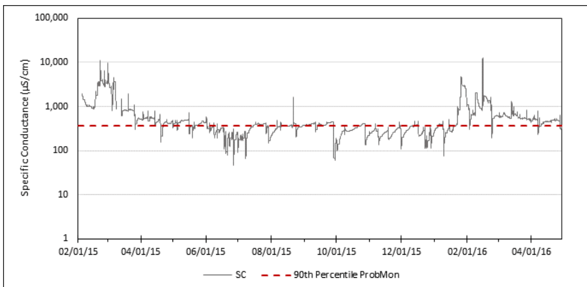
Figure 3-43: Observed Specific Conductance ( \mu\text{S/cm} ), Continuous Monitoring, Accotink Creek near Annandale
