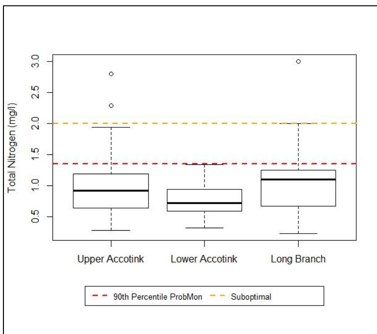
Figure 3-88: Ambient Total Nitrogen (mg/l) in Accotink Creek Watershed
