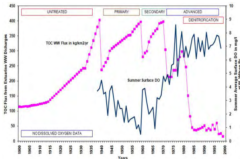
Figure 14. Total organic carbon from wastewater treatment plants and surface dissolved oxygen concentrations in the Potomac River tidal fresh estuary, at the Woodrow Wilson Bridge (Jaworski et al. 2007).
