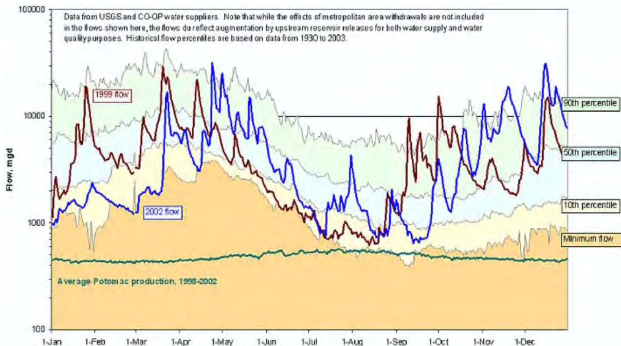
Figure 12. Adjusted Potomac River flows at Little Falls stream gage (USGS Station 01646502) in drought years.
