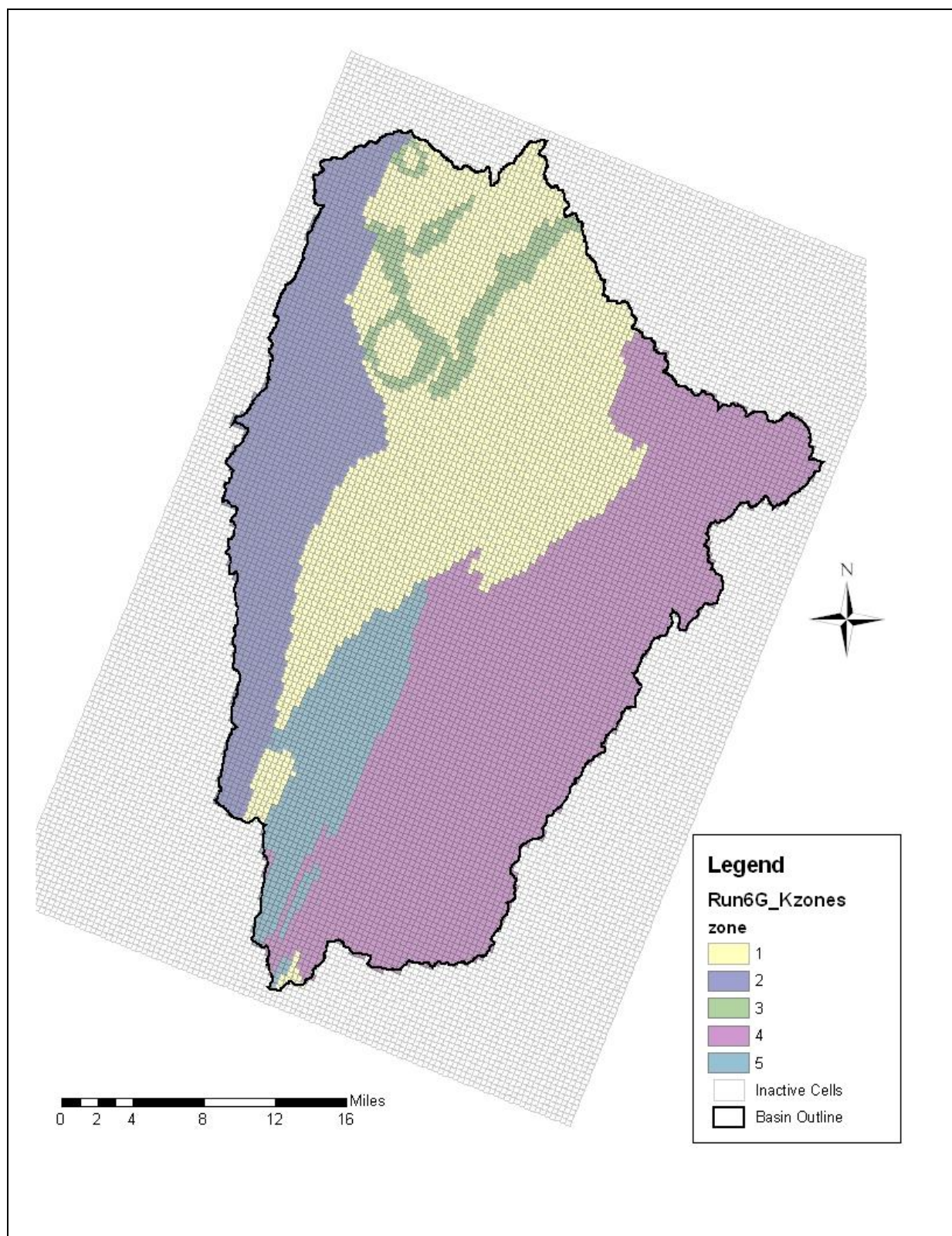
Figure 6. Model hydraulic conductivity zones.
