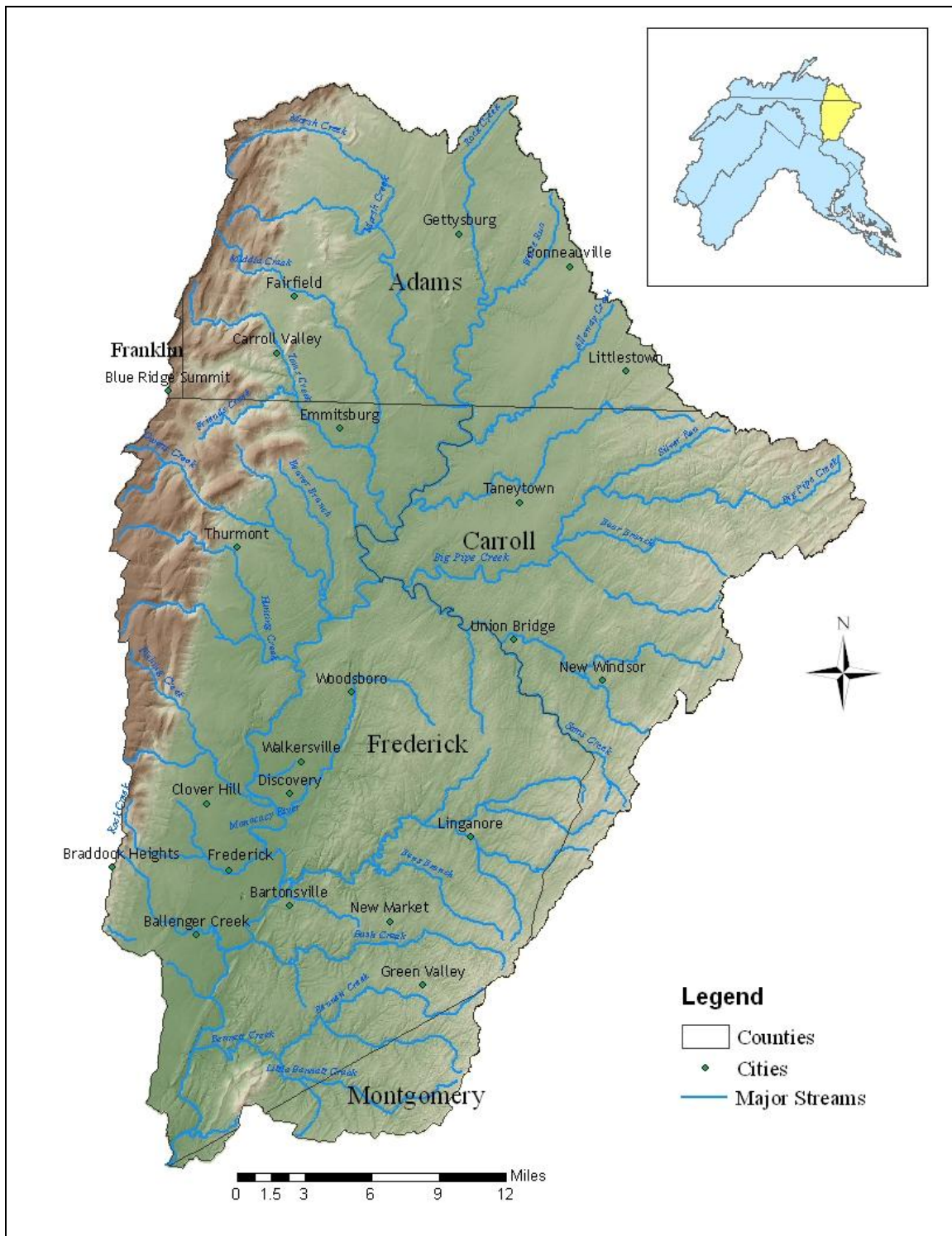
Figure 2. Geographic features, counties, and municipalities of the Monocacy basin
