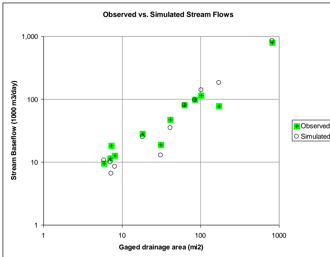
Figure 9. Observed versus simulated stream base flows for the year, 1980
