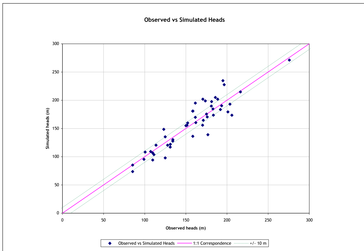
Figure 8. Observed versus simulated heads
