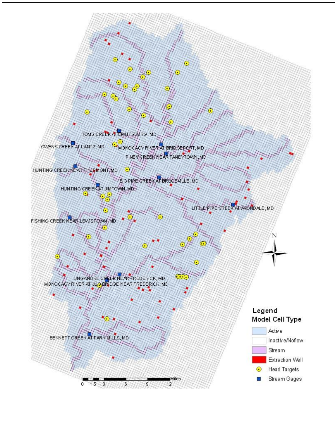
Figure 4. Model grid, with locations of stream and extraction well cells, water level targets, and stream gages.
