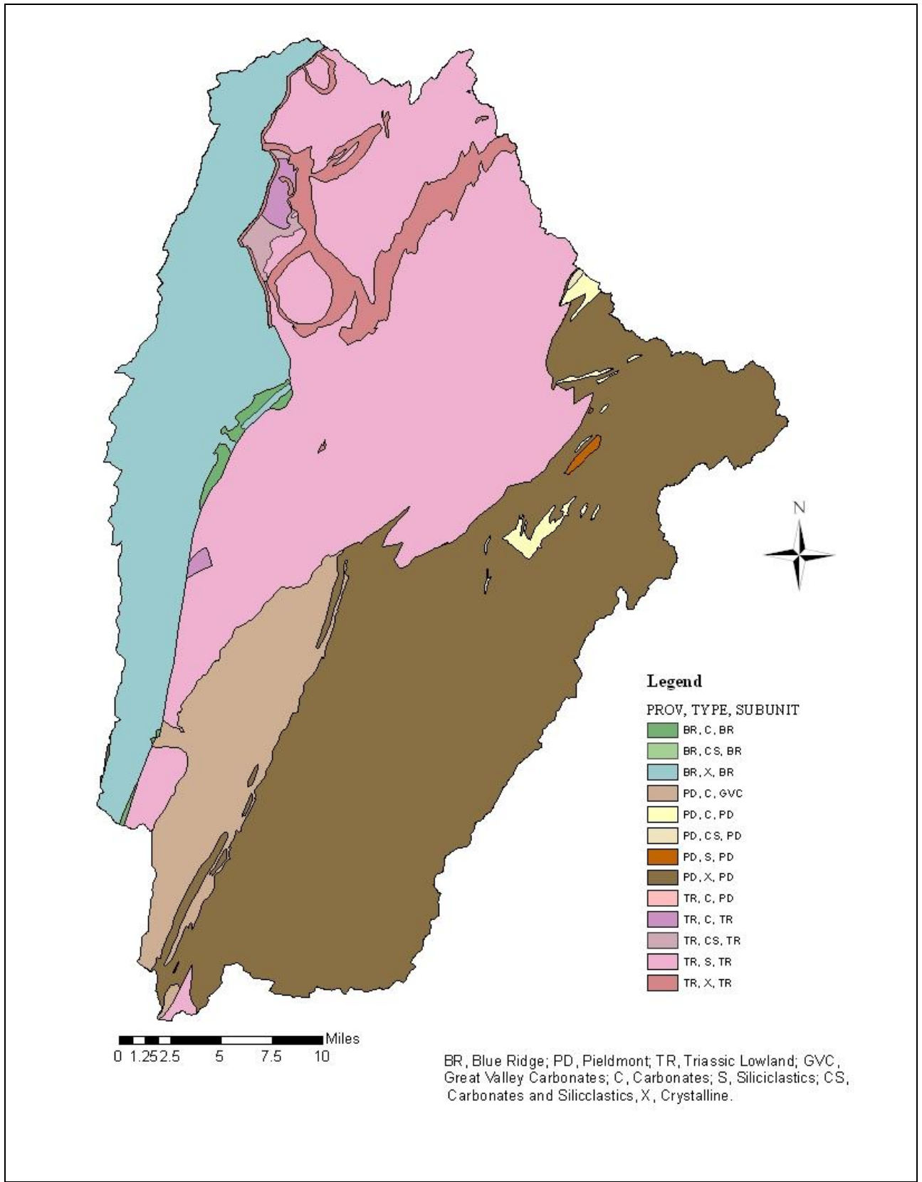
Figure 3. Geologic units in the Monocacy River basin (Derosier and others, 1998).
