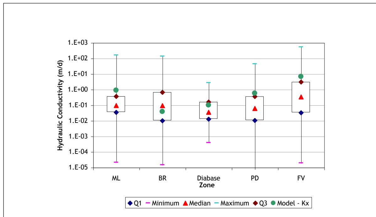
Figure 7. Comparisons of model hydraulic conductivities with values derived from well data
